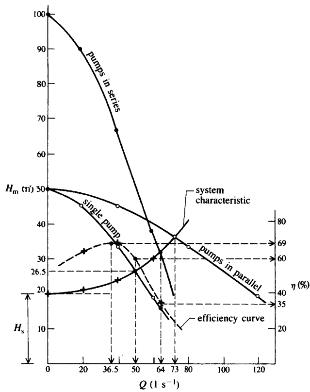
Fig. 13.14 Pump-pipeline characteristics
