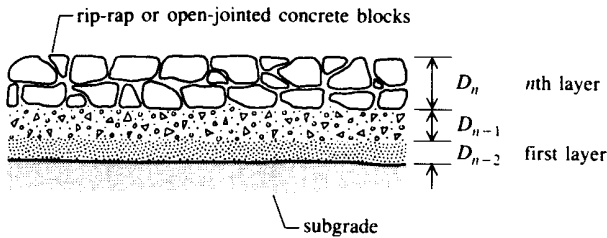
Fig. 9.11 Filter construction
