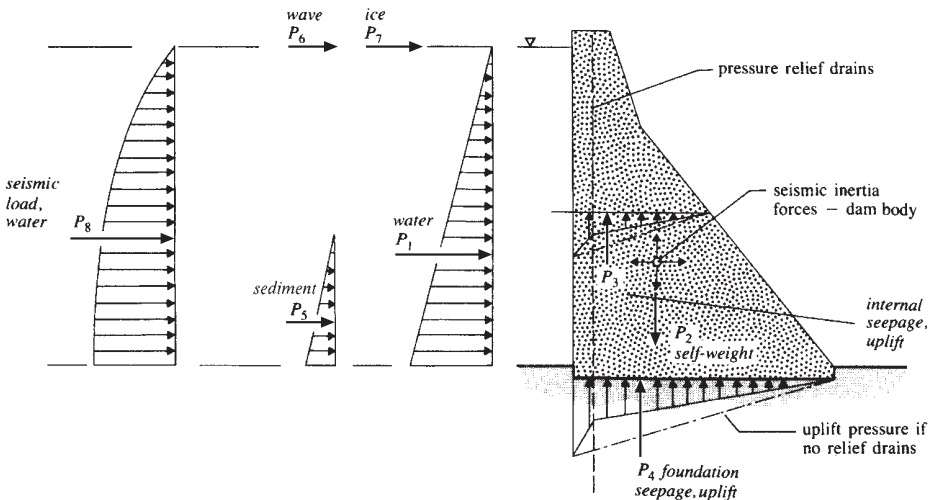
Fig. 1.8 Schematic of principal loads: gravity dam profile
