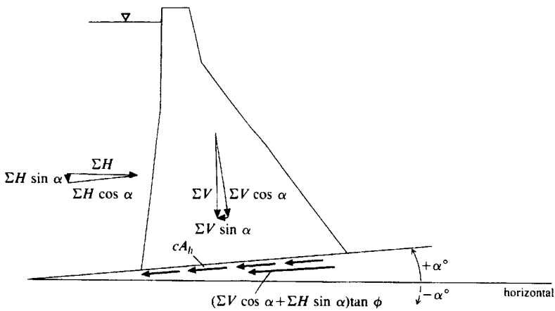
Fig. 3.5 Sliding and shearing resistance: shear friction factor
