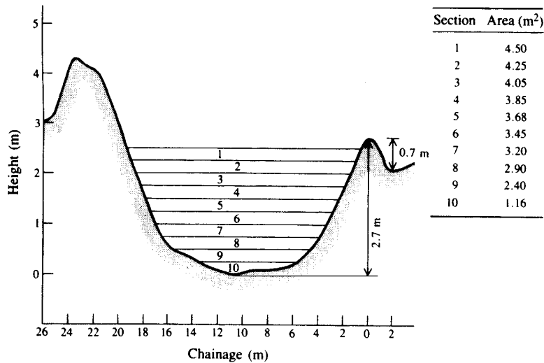
Fig. 8.21 River cross-section
